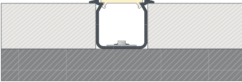
The mounting effect for the SKAGEN set in a milled hole.
