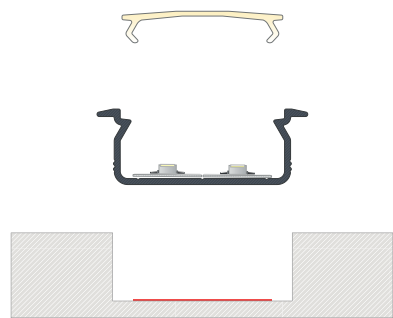
Assembly instructions for the TVED set in a milled hole using double-sided tape.
