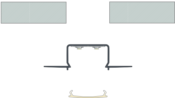
Assembly instructions of the HORST set between two plasterboards.
