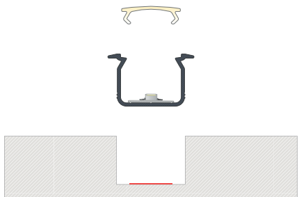
Assembly instructions for the UHRE set in a milled hole using double-sided tape.
