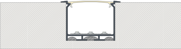
The mounting effect for the HEDE set in a milled hole using mounting adhesive.
