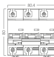
MCB-3P
