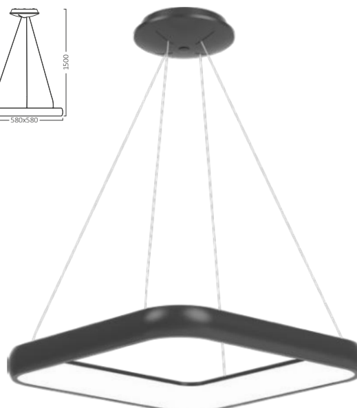
Bella BH17-03981 3CCT 46W 5200lm Black 220-240V CRI>80 IP20 Aluminium 3CCT
