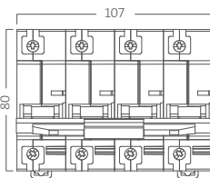
MCB-4P
